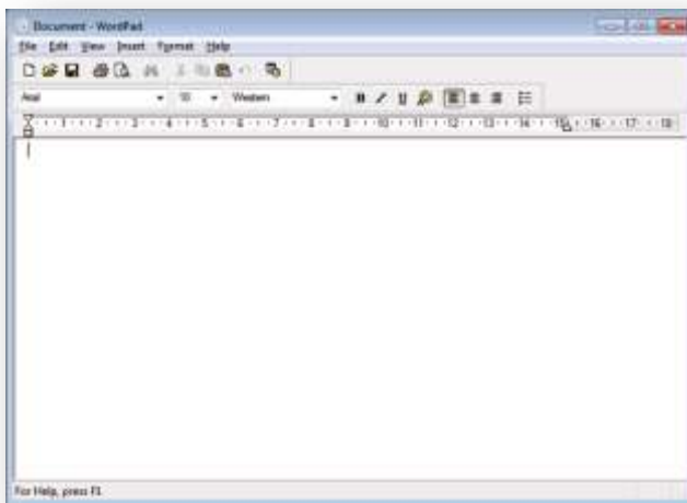
WORDPAD
